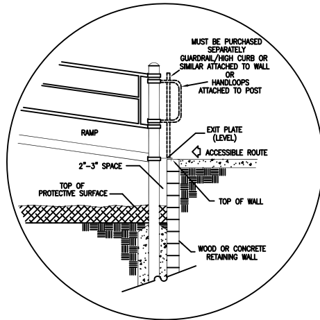
SUGGESTED ELEVATED RAMP EXIT INSTALLATION RAMP ELEVATION TO BE 32" ABOVE FINISH GRADE.
